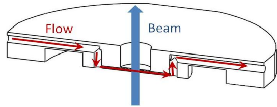
Fig. 3. FAST microfluidics chip cross section.
