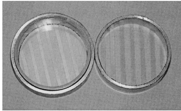
FIG. 1. Double ring Mylar dishes used for bystander studies. Left: Photograph shows the outer stainless steel ring with a base made of Mylar that is 6 \mu\text{m} thick, and contained within is the inner ring bearing several strips of 30- \mu\text{m} Mylar as a base. The outer and inner rings fit together. Right: The inner ring with strips of Mylar.
